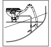
Toilet mounted above the waterline and discharging overboard.
