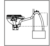
Toilet waste discharging into holding tank, discharging elbow always above top of the holding tank.
