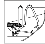
Toilet mounted below the waterline and discharging overboard.
