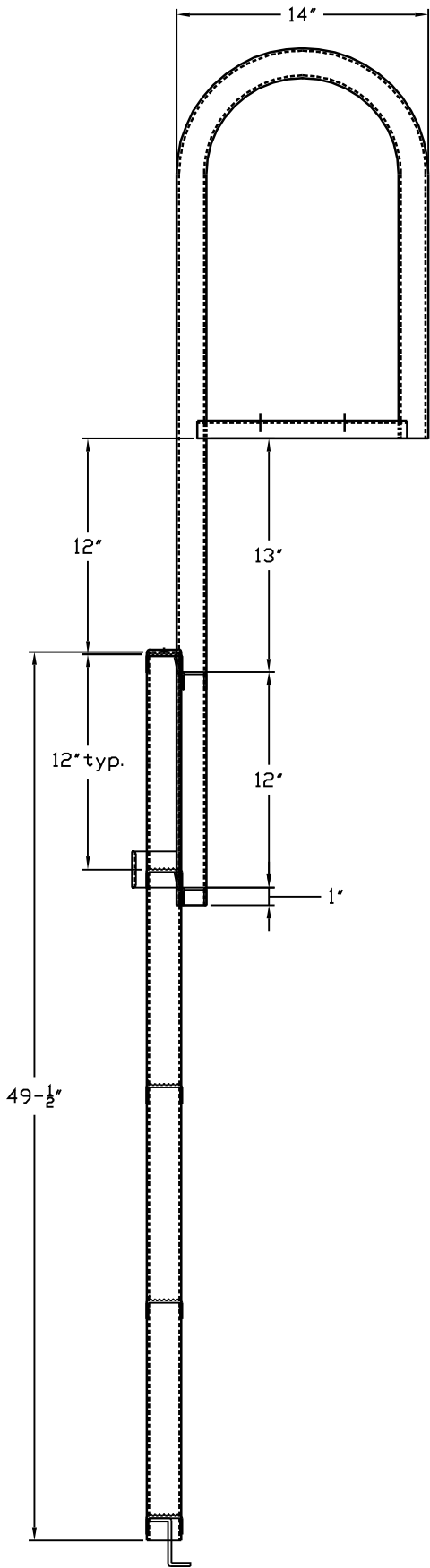
VIEW IN DOWN POSITION
