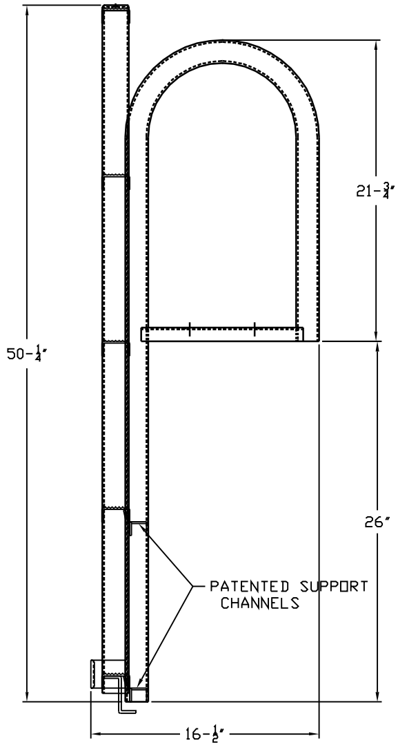
VIEW IN UP POSITION
