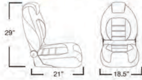
Seat Dimensions
