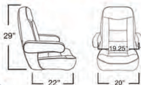
Seat Dimensions
