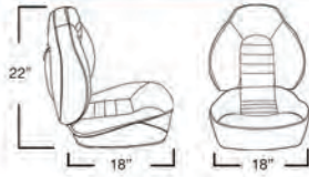
Seat Dimensions
