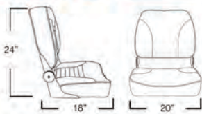
Seat Dimensions
