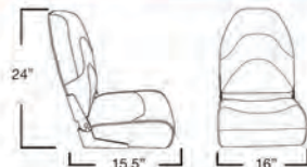
Seat Dimensions
