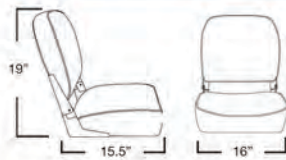
Seat Dimensions
