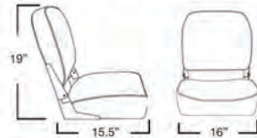
Seat Dimensions
