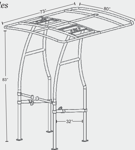
Footprint dims: 39-1/2" L x 18" to 51" W (adj.)
