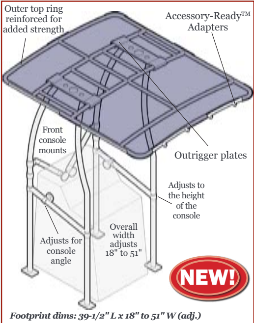
Footprint dims: 39-1/2" L x 18" to 51" W (adj.)
