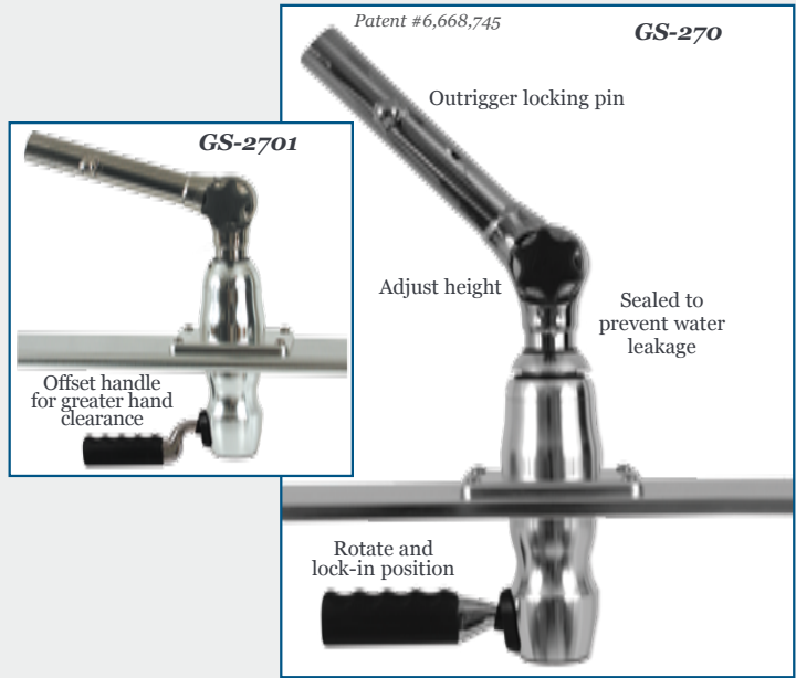
Variable Rotator Handle Installation Positioning
