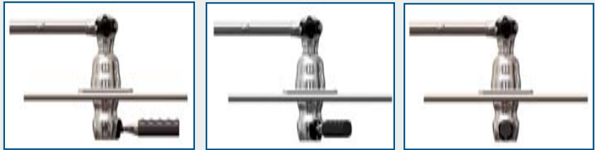
Variable Rotator Handle Installation Positioning
