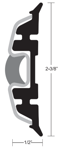
Assembled View
