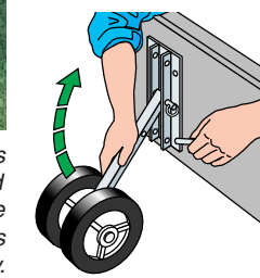
Removal of the two lower lockpins allows the wheels to be pivoted and locked in an upright position while underway. Removal of all four pins releases the entire wheel assembly.
